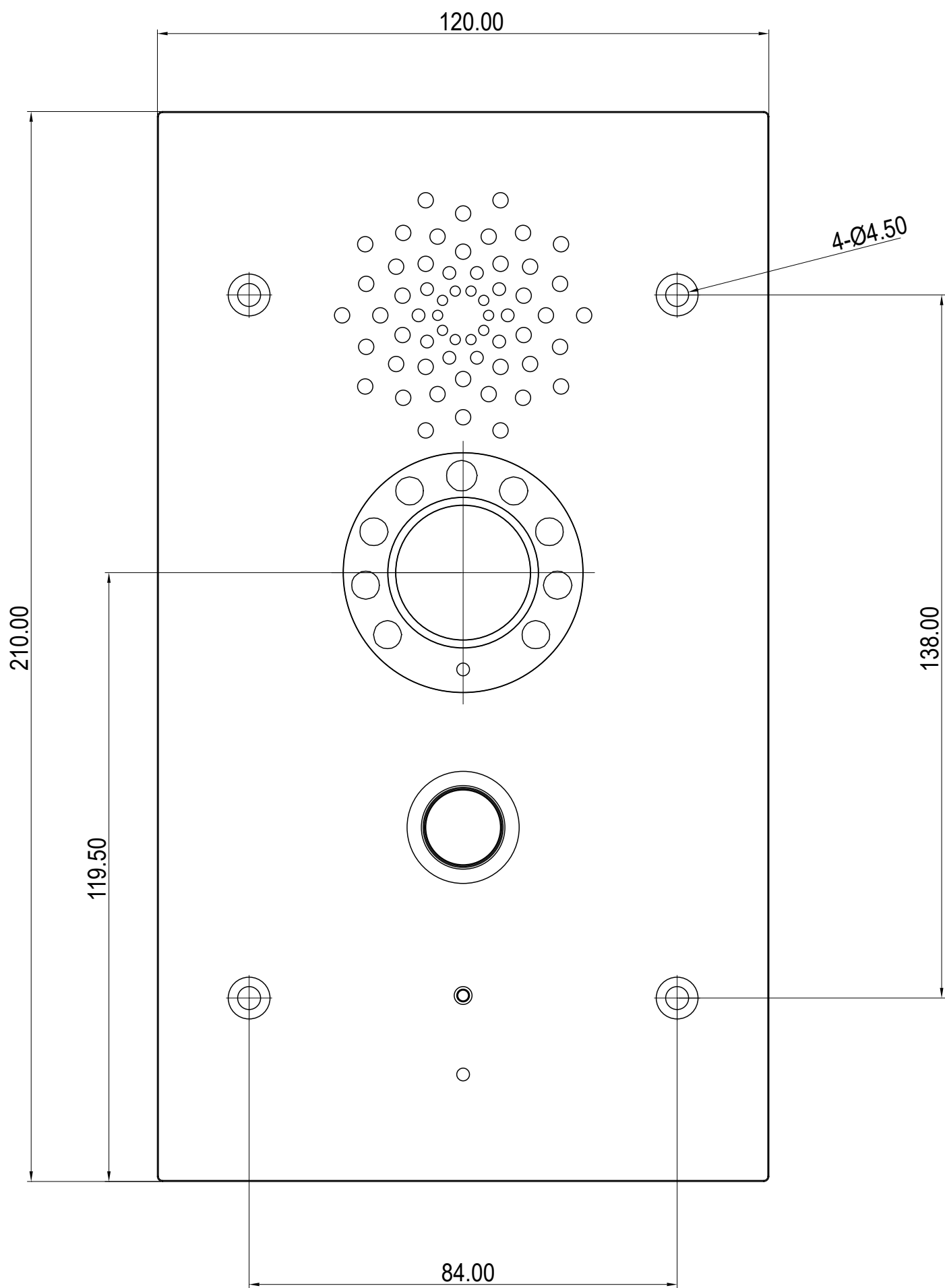
1 FRONT VIEW
