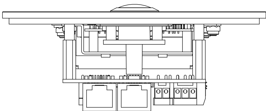
6 BOTTOM VIEW
