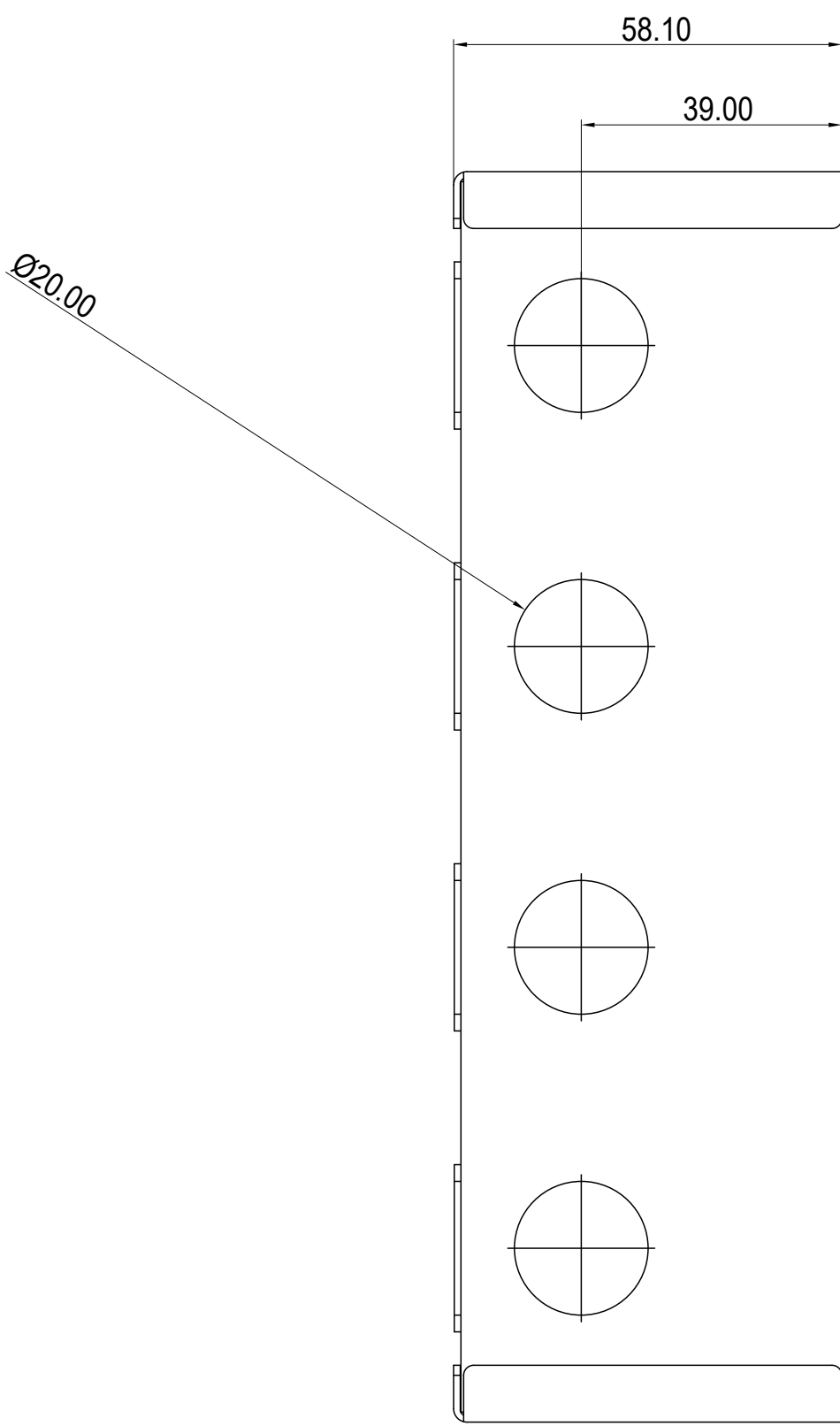
2 RIGHT VIEW
