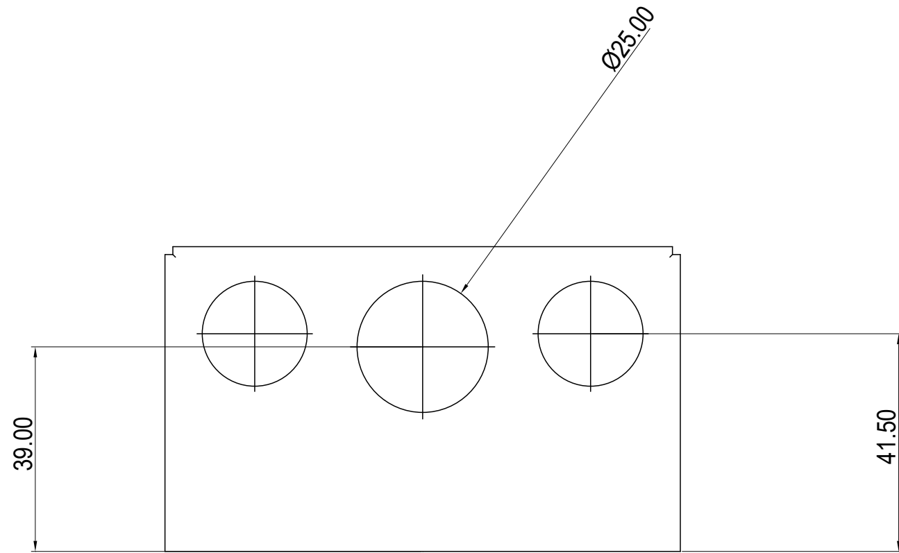
5 TOP VIEW
