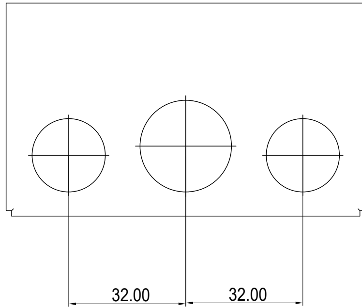
6 BOTTOM VIEW
