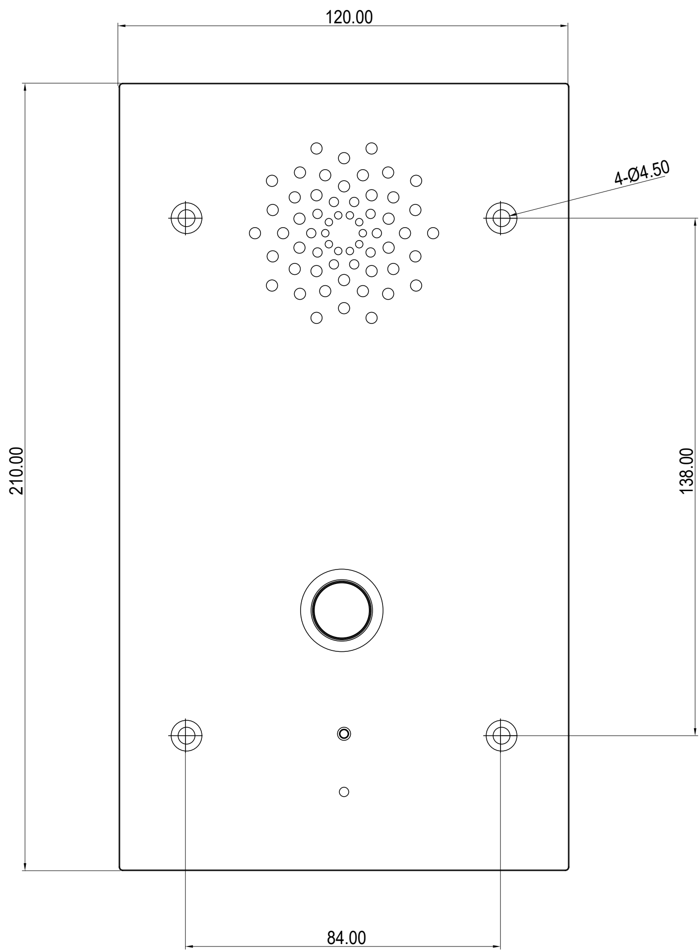
1 FRONT VIEW
