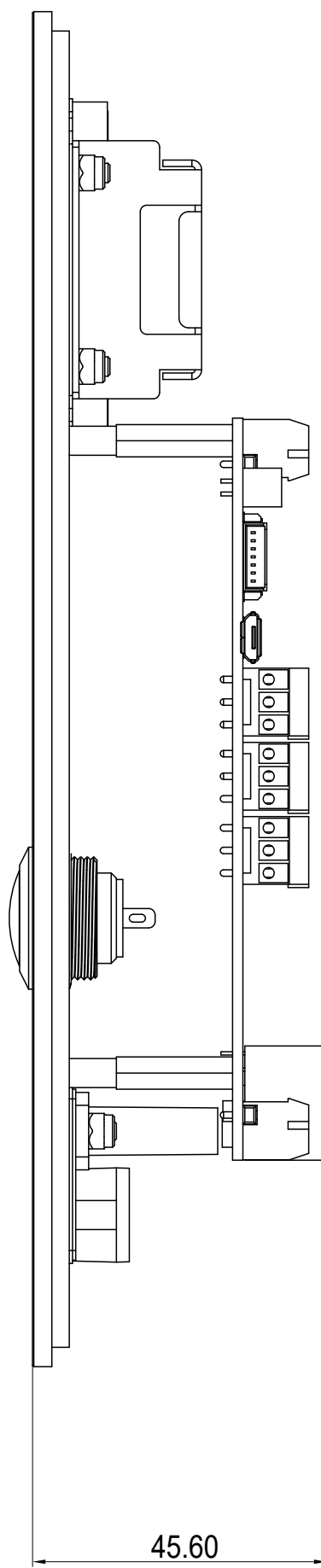
3 LEFT VIEW
