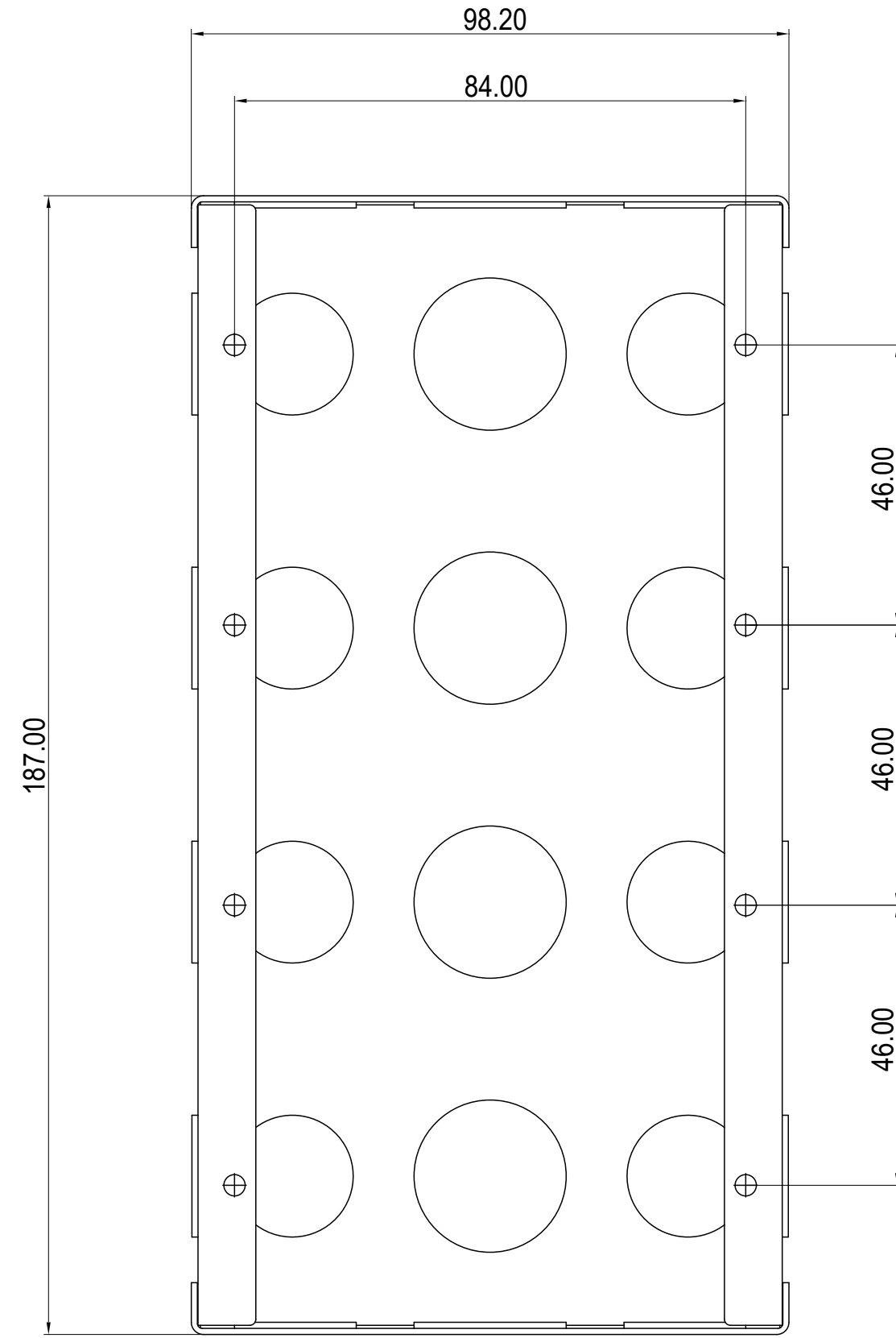
1 FRONT VIEW
