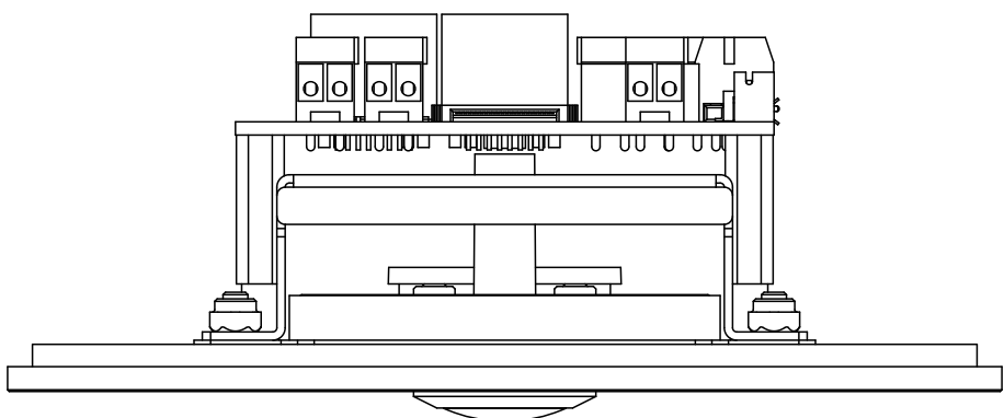
5 TOP VIEW
