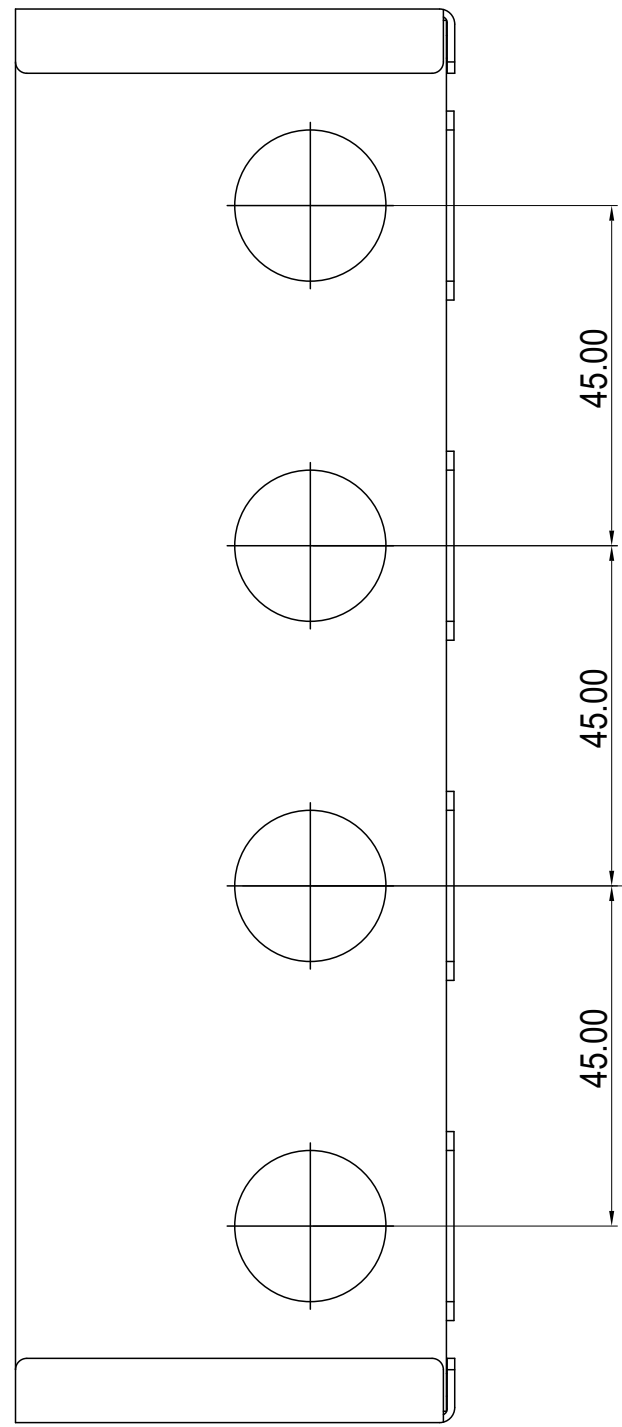
3 LEFT VIEW
